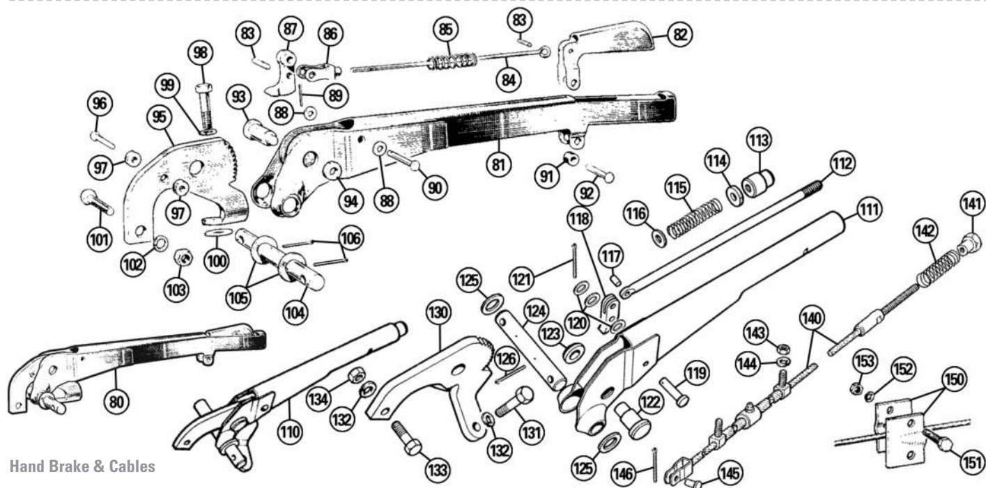
Rear Brakes
