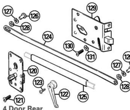
4 Door Rear
