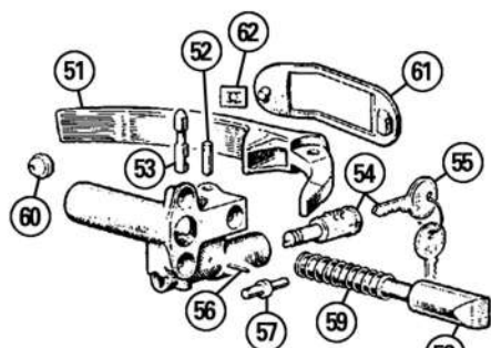
2 Door External Locking (Early)
