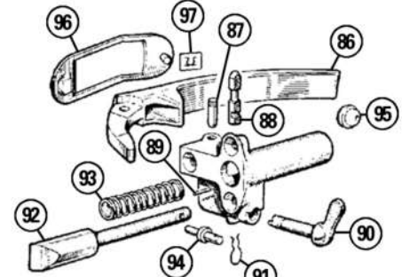
2 Door Internal Locking
