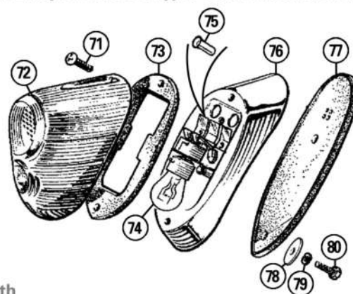
Stop & Tail Lamp: Lucas 549 Type, With Chrome Plinth
