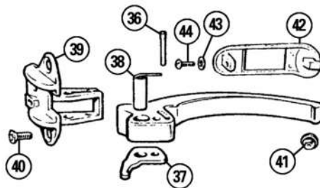
4 Door Rear
