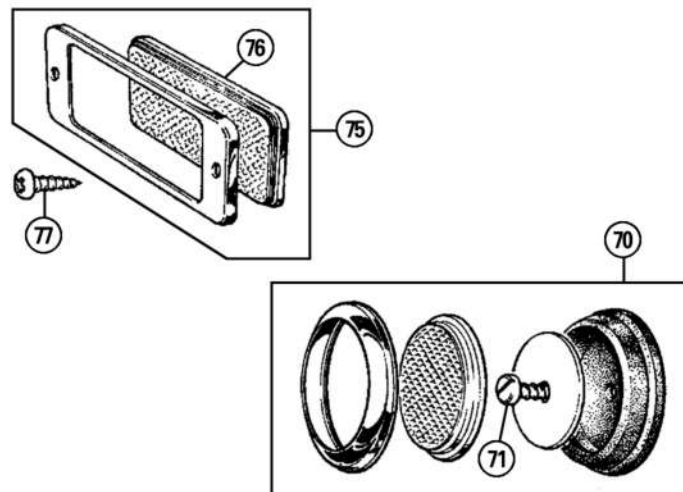
Reflectors
