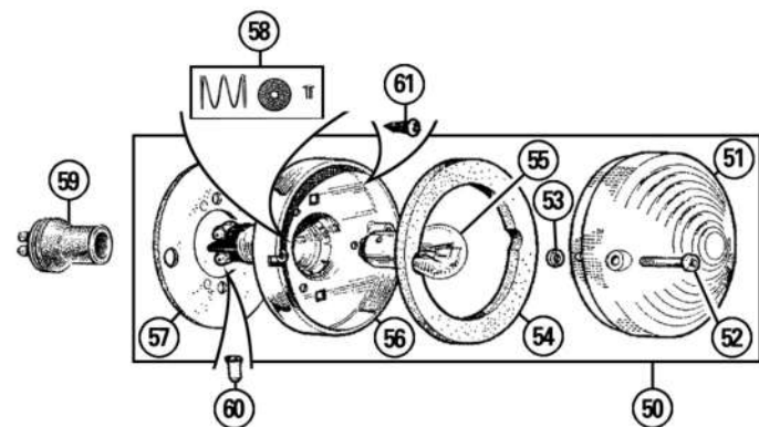
Indicator Lamp: Lucas 491 Type - Traveller (from (c) NAS 1075912)
